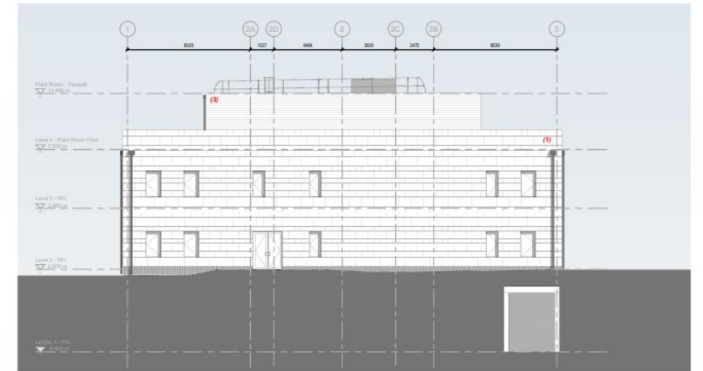
④ South - Elevation - Facing Keith Day Road 1:100
