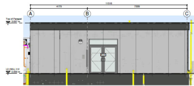
West Elevation 1:50
